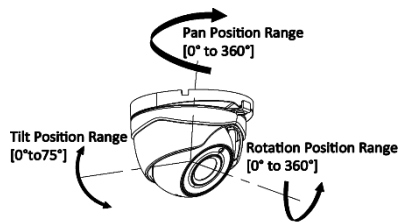
Figure 2-14 3-axis Adjustment
