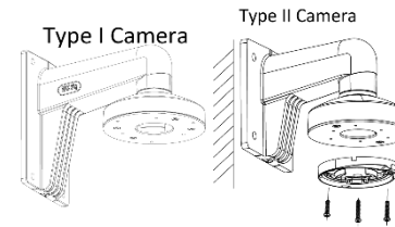
Figure 2-17 Install the Pendant Bracket
