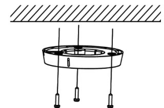
Figure 2-3 Attach the Mounting Base to the Ceiling
