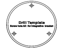
Figure 2-11 Drill Template
