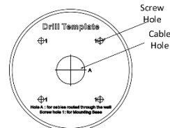
Figure 2-6 The Drill Template
