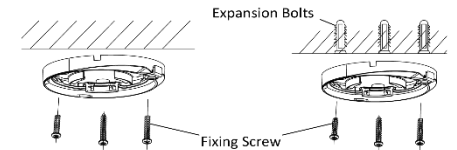
Figure 2-12 Fix the Mounting Base to the Ceiling
