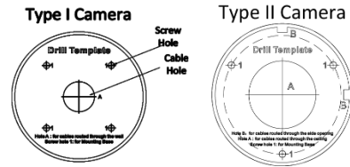
Figure 2-15 Drill Template of the Junction Box
