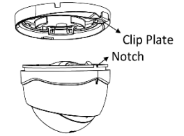
Figure 2-10 Disassemble the Camera
