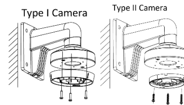
Figure 2-18 Install the Mounting Base to the Pendant Bracket
